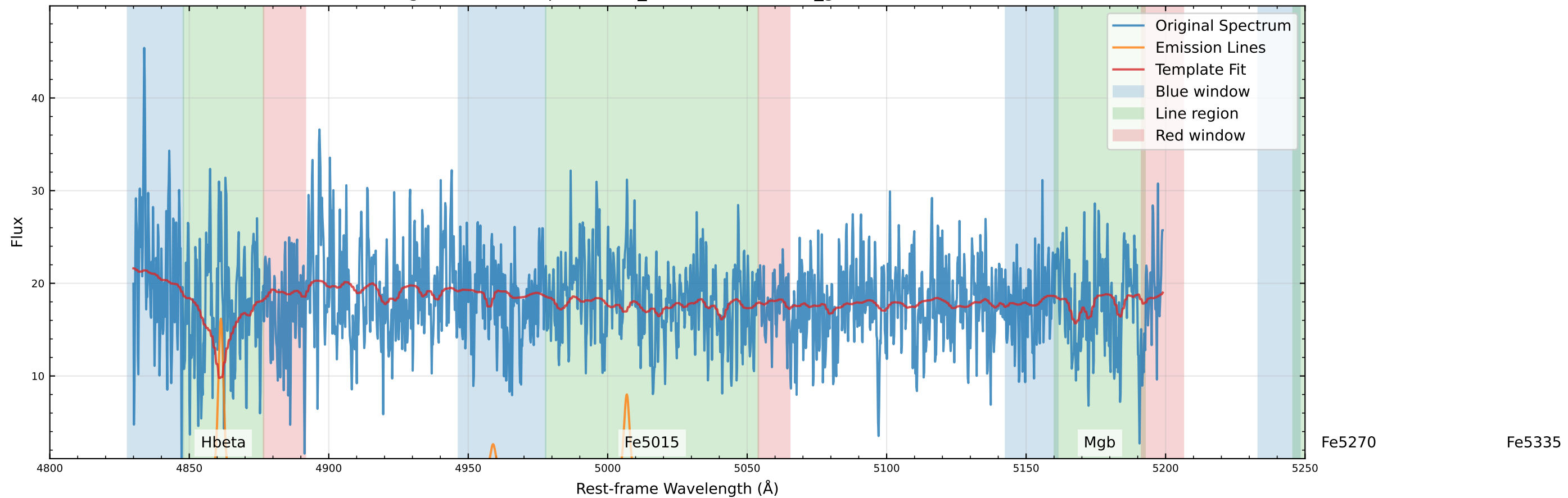
Original Data Comparison ( v_{\text{star}}=-36.9 km/s, v_{\text{gas}}=-17.6 km/s)
