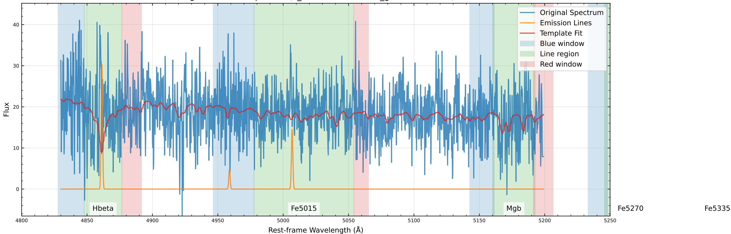
Original Data Comparison (v_star=-85.9 km/s, v_gas=-71.8 km/s)
