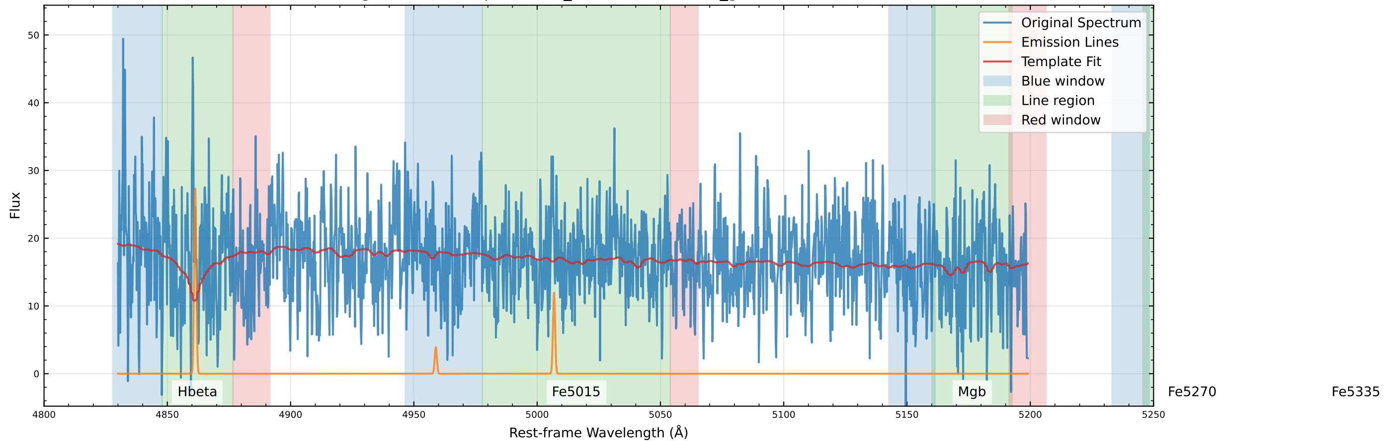
Original Data Comparison (v_star=-42.4 km/s, v_gas=-56.1 km/s)
