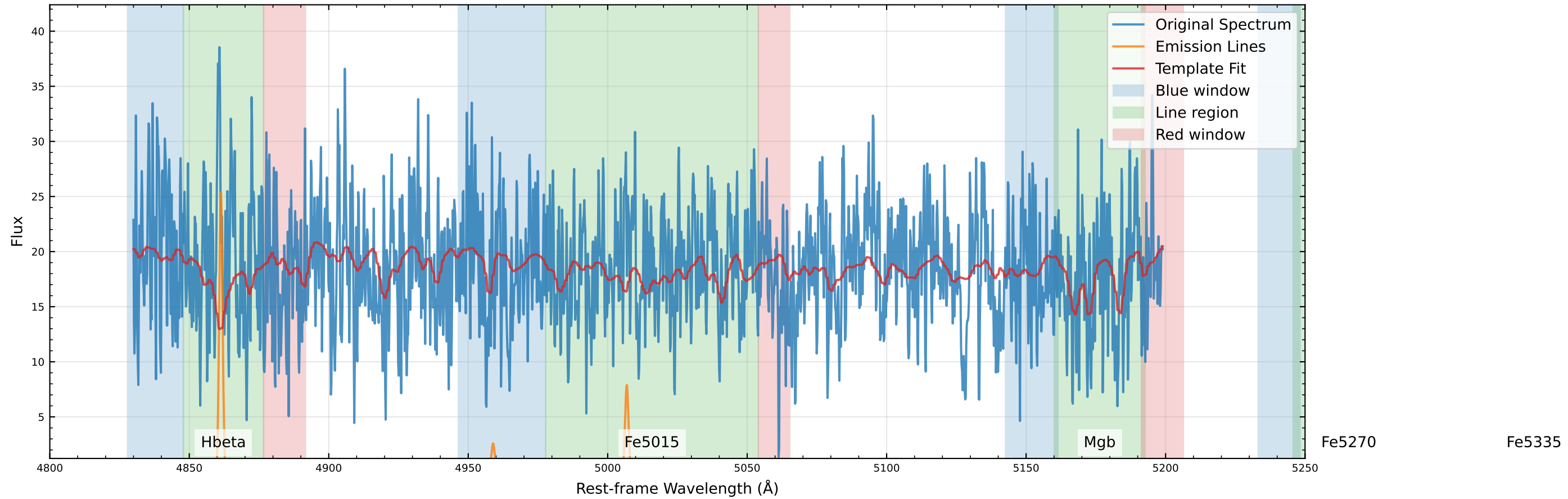
Original Data Comparison ( v_{\text{star}}=-32.8 km/s, v_{\text{gas}}=-44.2 km/s)
