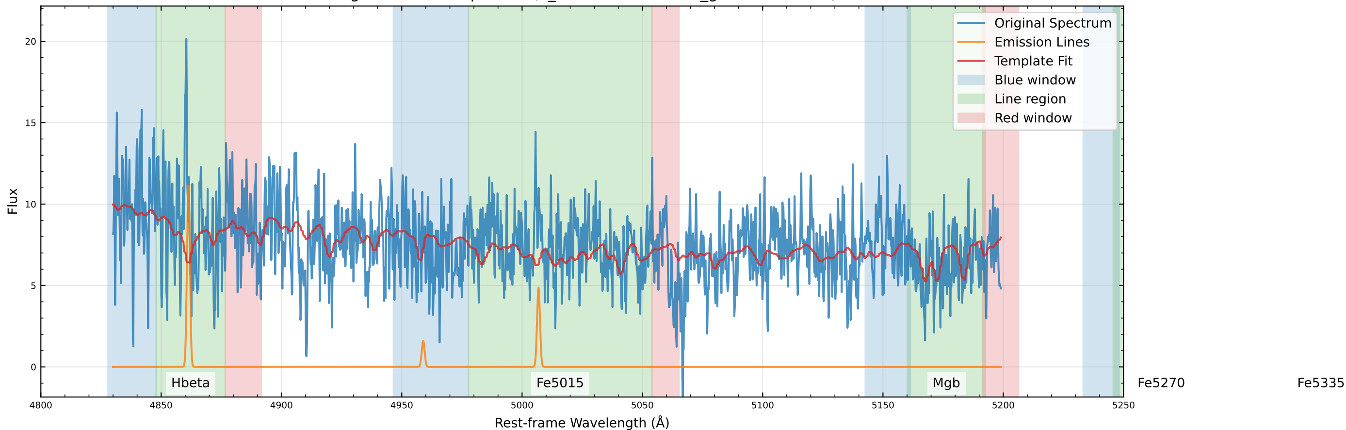
Original Data Comparison (v_star=-55.2 km/s, v_gas=-63.2 km/s)
