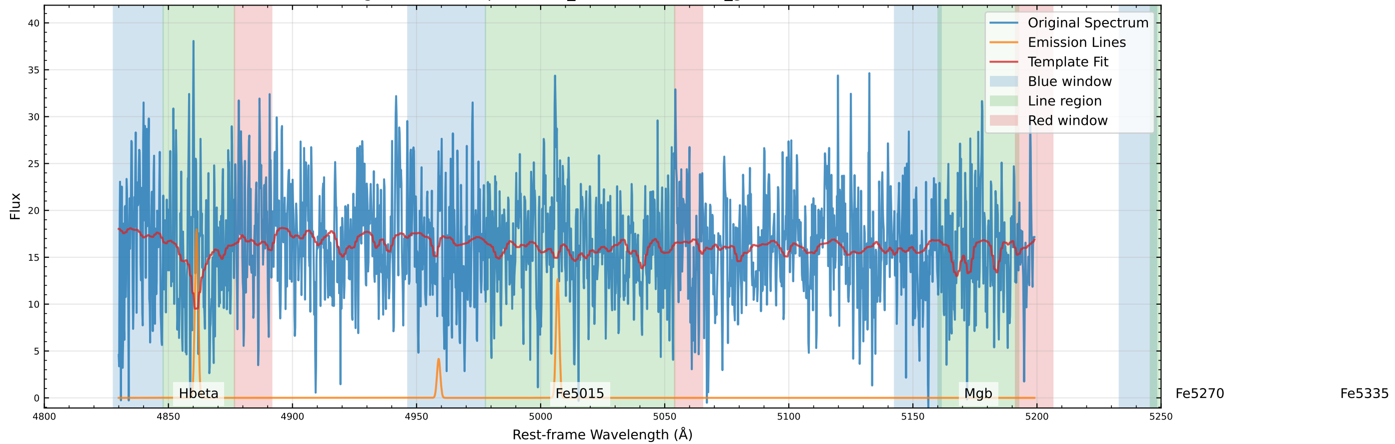
Original Data Comparison (v_star=-63.1 km/s, v_gas=-50.1 km/s)
