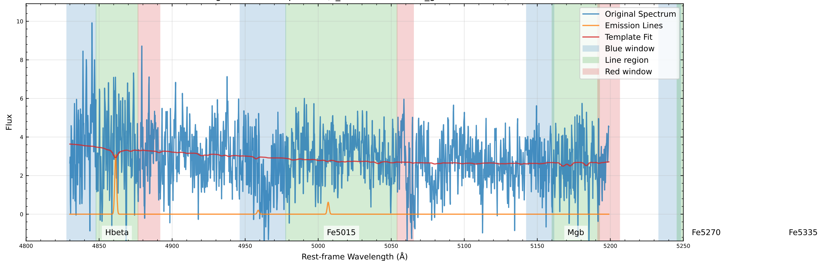
Original Data Comparison (v_star=37.4 km/s, v_gas=-29.4 km/s)
