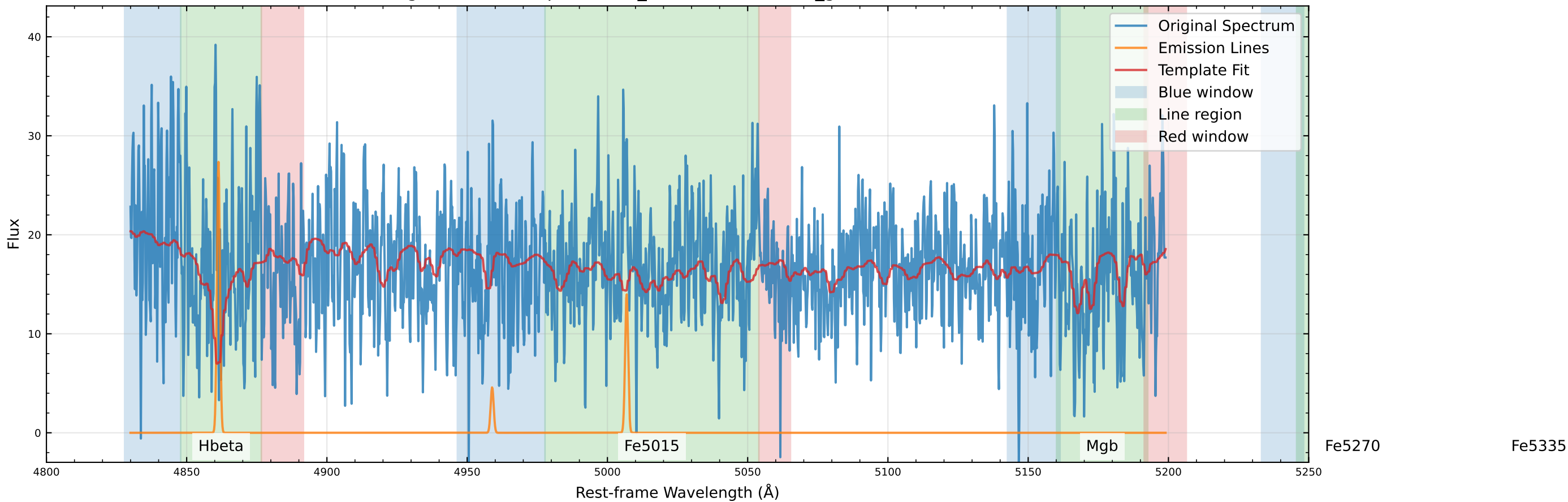
Original Data Comparison (v_star=-64.2 km/s, v_gas=-63.1 km/s)
