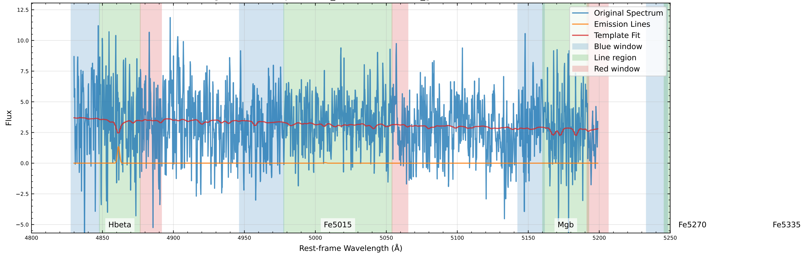
Original Data Comparison (v_star=-52.9 km/s, v_gas=-63.7 km/s)
