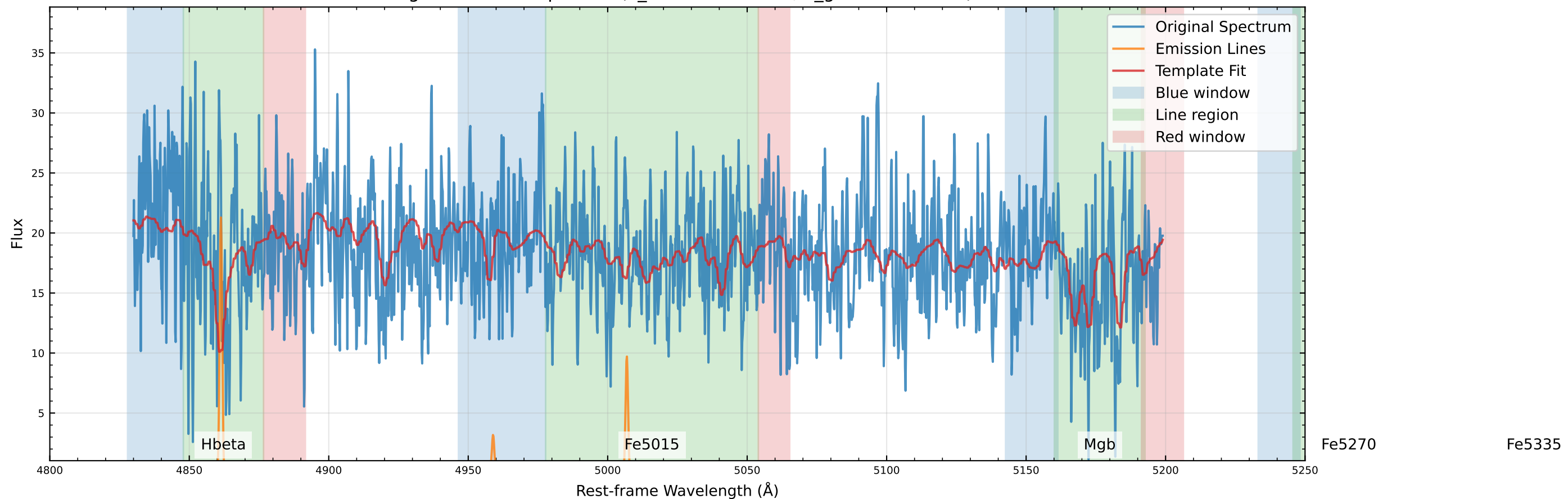
Original Data Comparison (v_star=-52.2 km/s, v_gas=-30.9 km/s)
