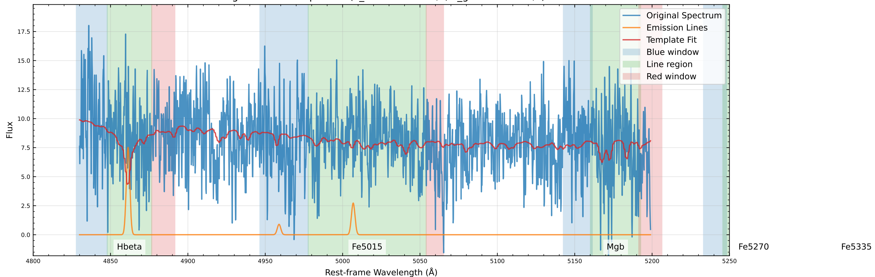
Original Data Comparison (v_star=-73.3 km/s, v_gas=-96.8 km/s)
