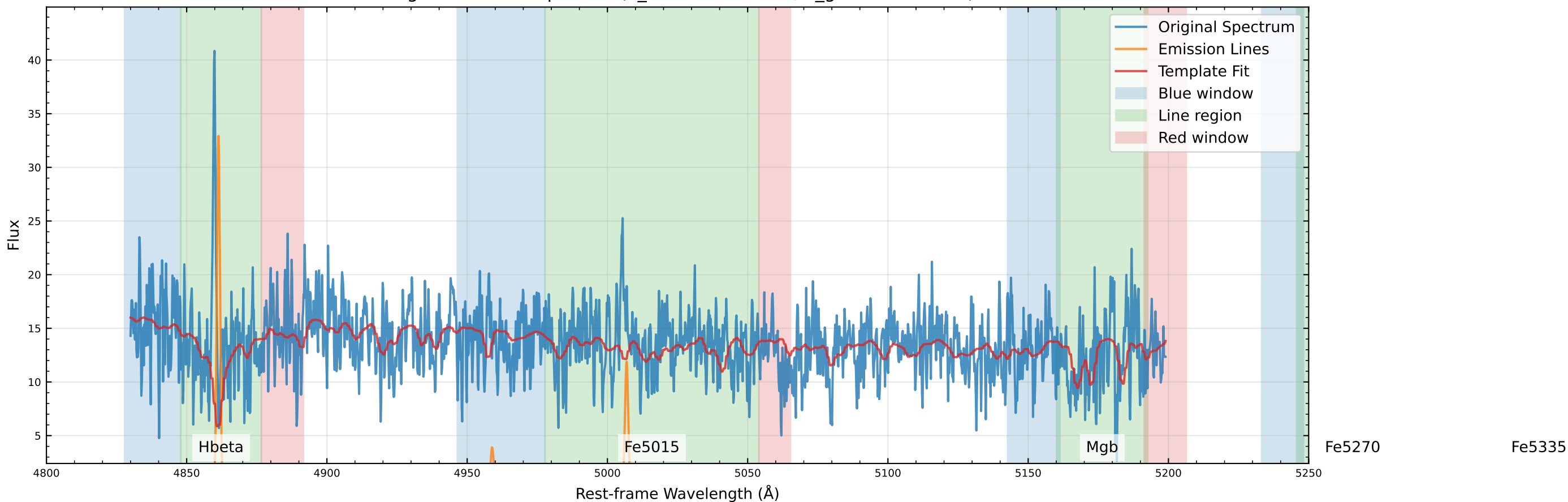
Original Data Comparison (v_star=-75.0 km/s, v_gas=-91.8 km/s)
