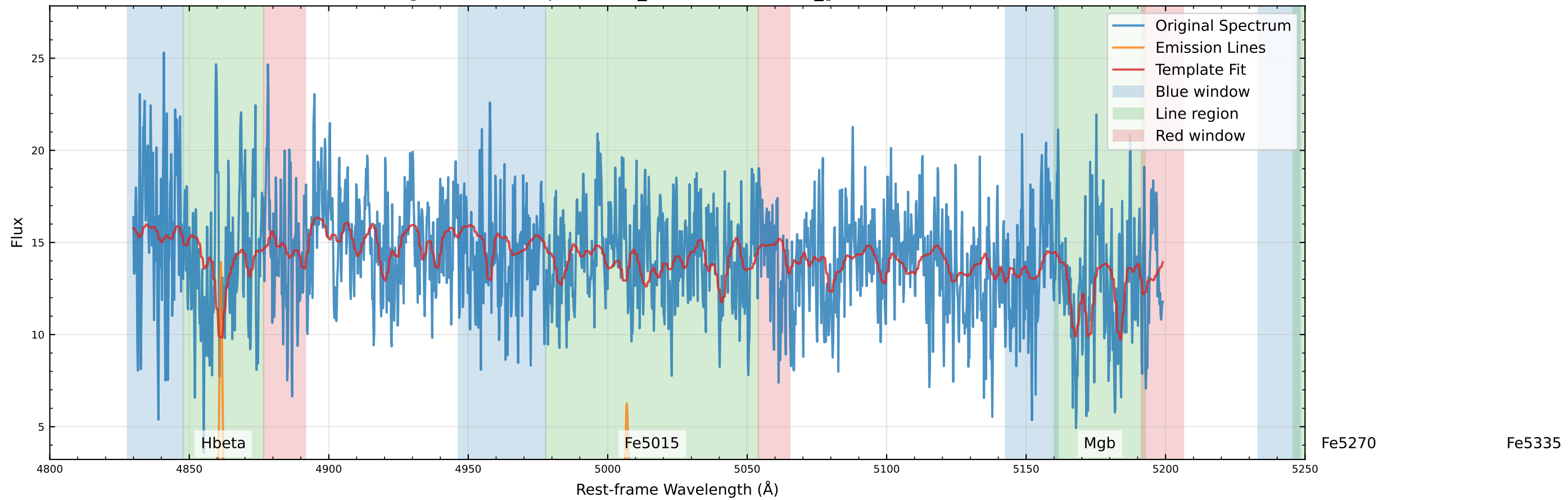
Original Data Comparison (v_star=-67.5 km/s, v_gas=-92.5 km/s)
