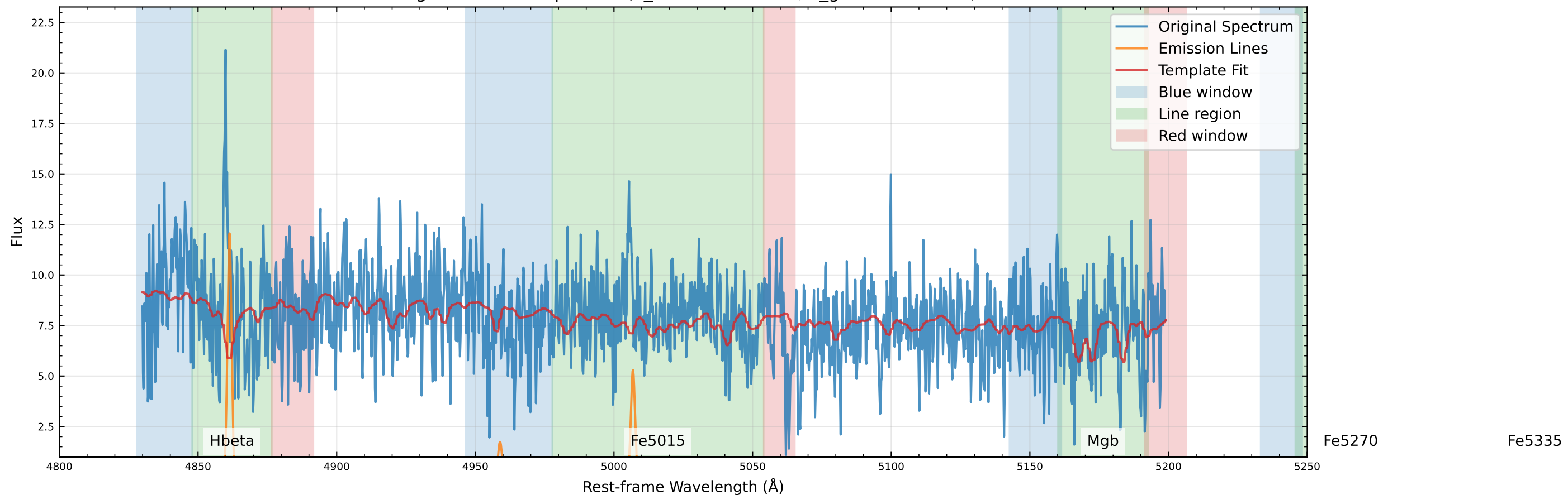
Original Data Comparison (v_star=-81.7 km/s, v_gas=-86.3 km/s)
