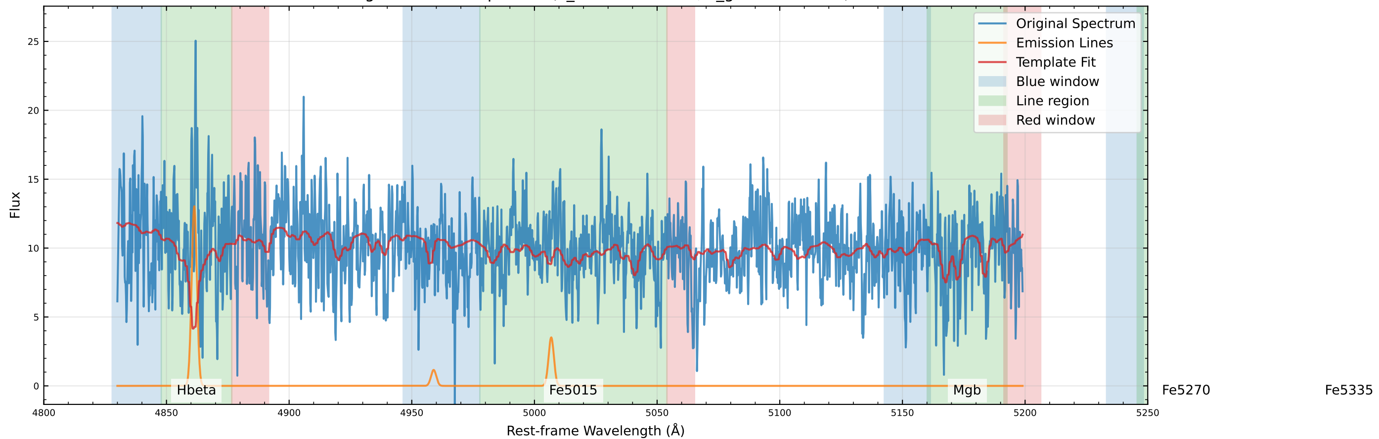
Original Data Comparison (v_star=35.3 km/s, v_gas=26.3 km/s)
