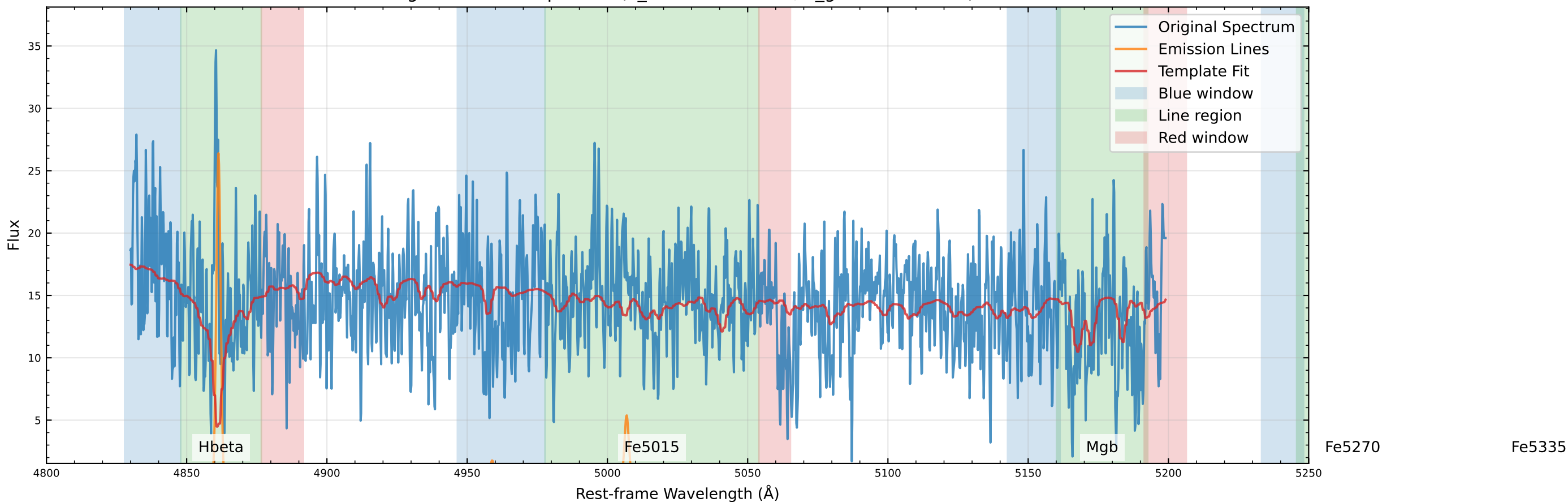
Original Data Comparison (v_star=-87.3 km/s, v_gas=-58.1 km/s)
