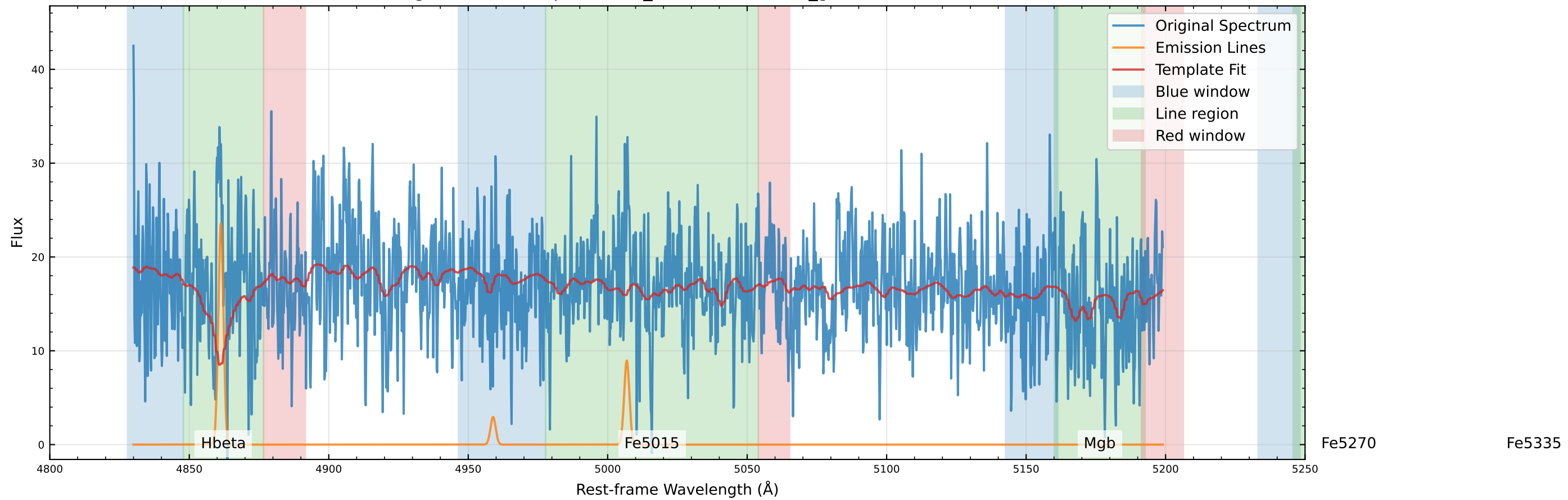
Original Data Comparison (v_star=-0.0 km/s, v_gas=-21.0 km/s)
