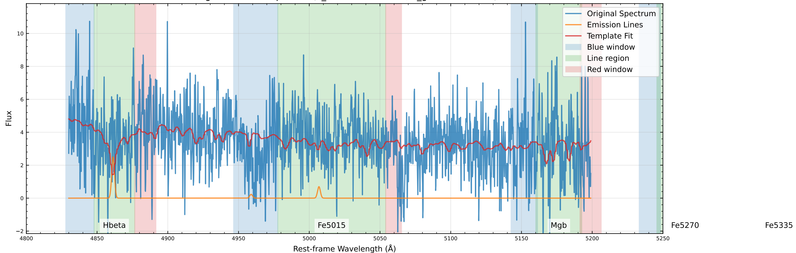
Original Data Comparison (v_star=-134.1 km/s, v_gas=-84.1 km/s)
