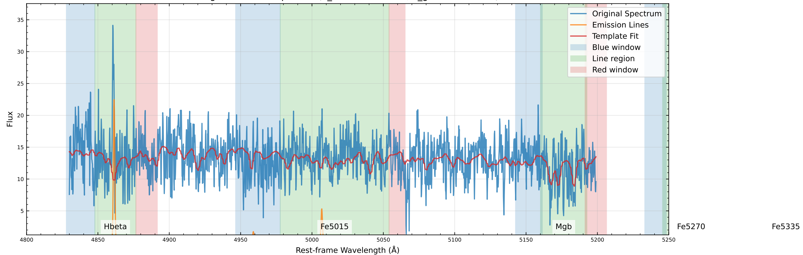
Original Data Comparison (v_star=-22.5 km/s, v_gas=-37.5 km/s)
