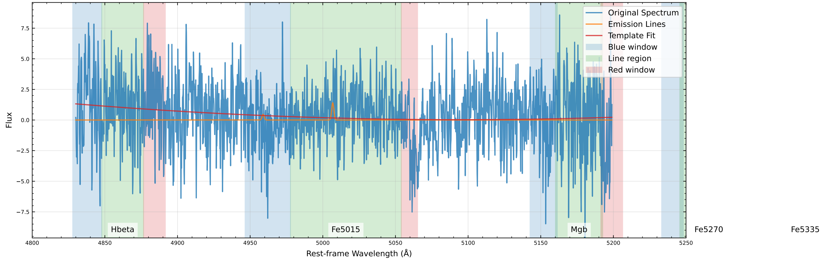
Original Data Comparison (v_star=3.3 km/s, v_gas=62.6 km/s)
