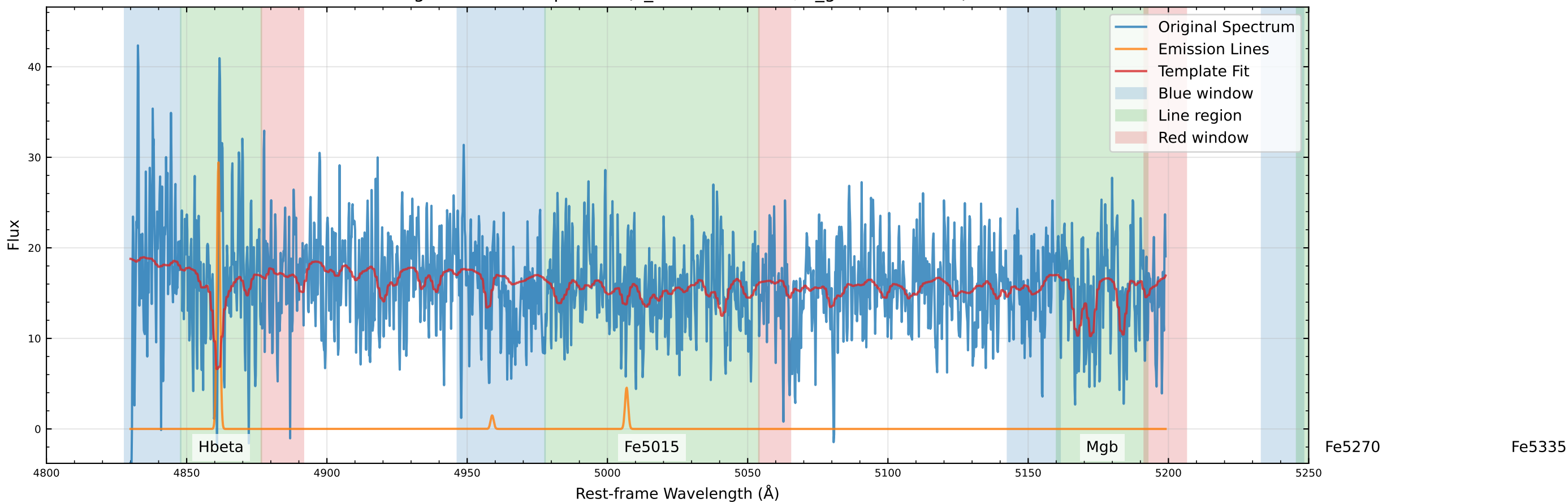
Original Data Comparison (v_star=38.5 km/s, v_gas=42.1 km/s)
