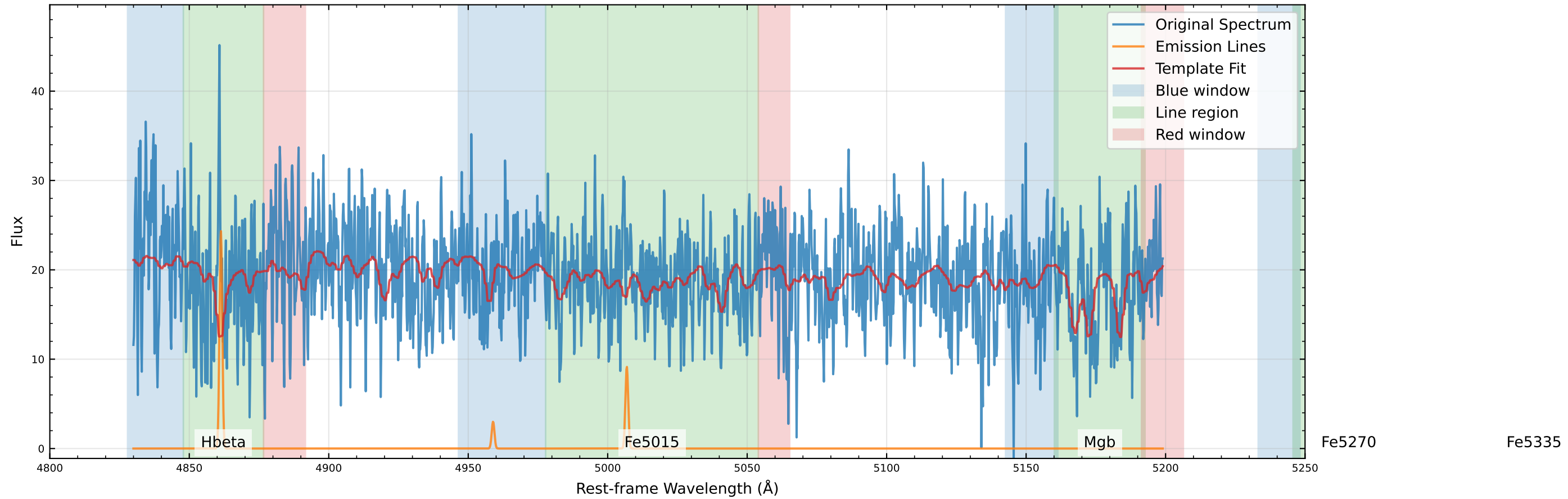
Original Data Comparison (v_star=-27.3 km/s, v_gas=-40.0 km/s)
