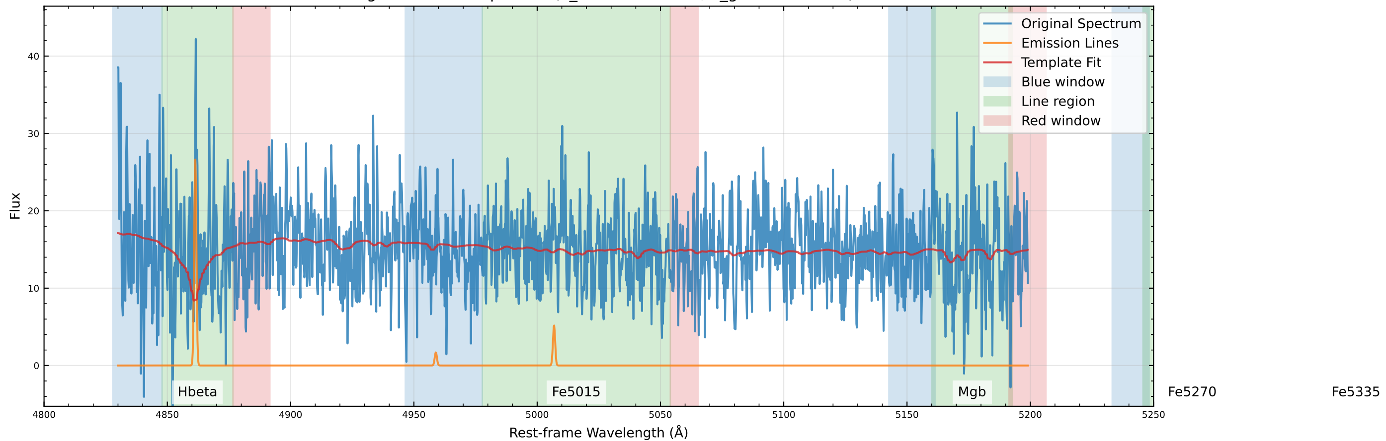
Original Data Comparison (v_star=22.2 km/s, v_gas=21.2 km/s)
