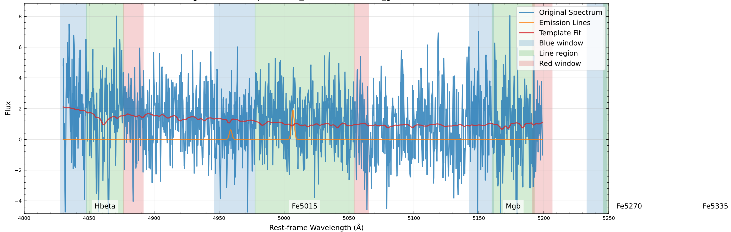
Original Data Comparison (v_star=-70.2 km/s, v_gas=22.0 km/s)
