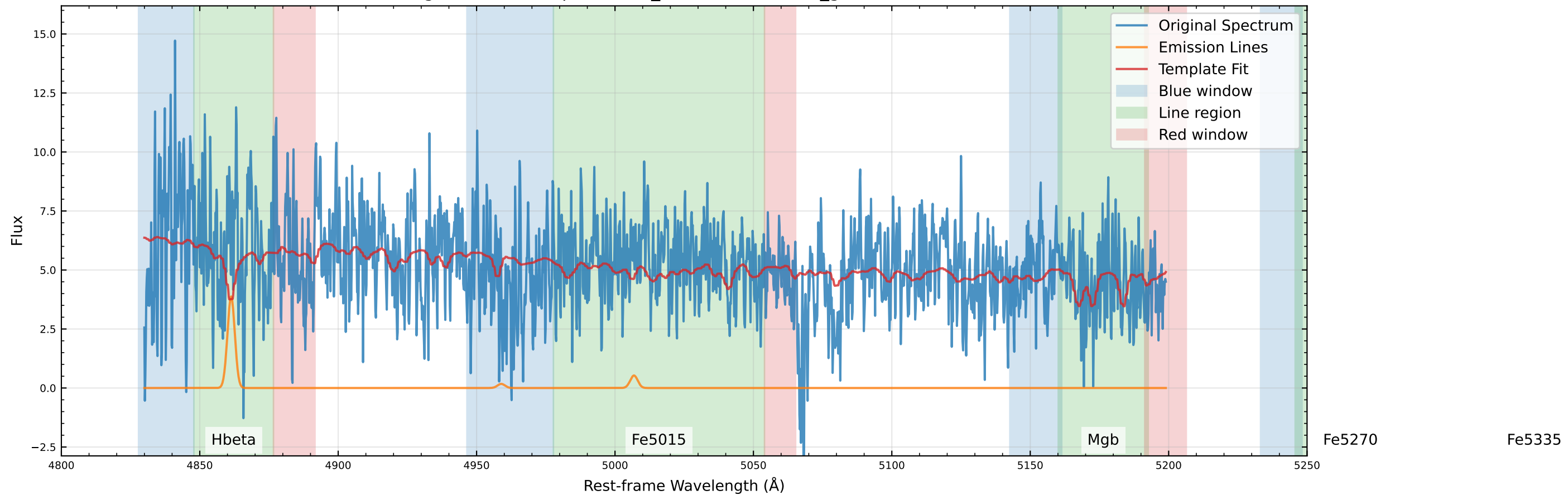
Original Data Comparison (v_star=32.1 km/s, v_gas=51.9 km/s)
