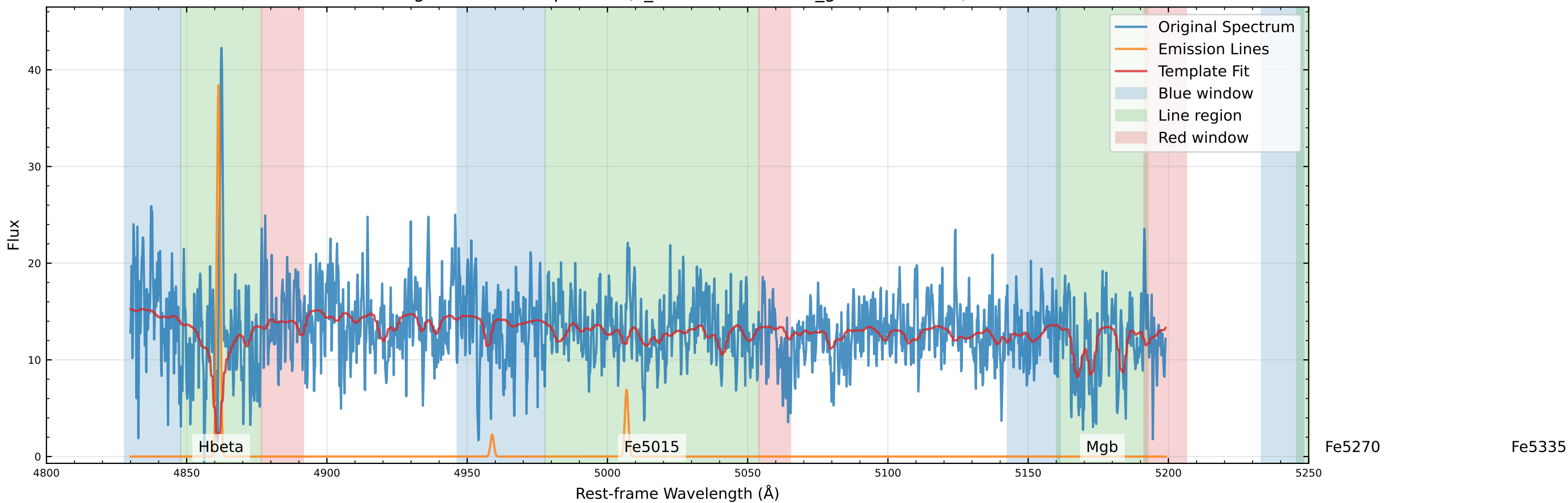
Original Data Comparison (v_star=51.1 km/s, v_gas=61.7 km/s)
