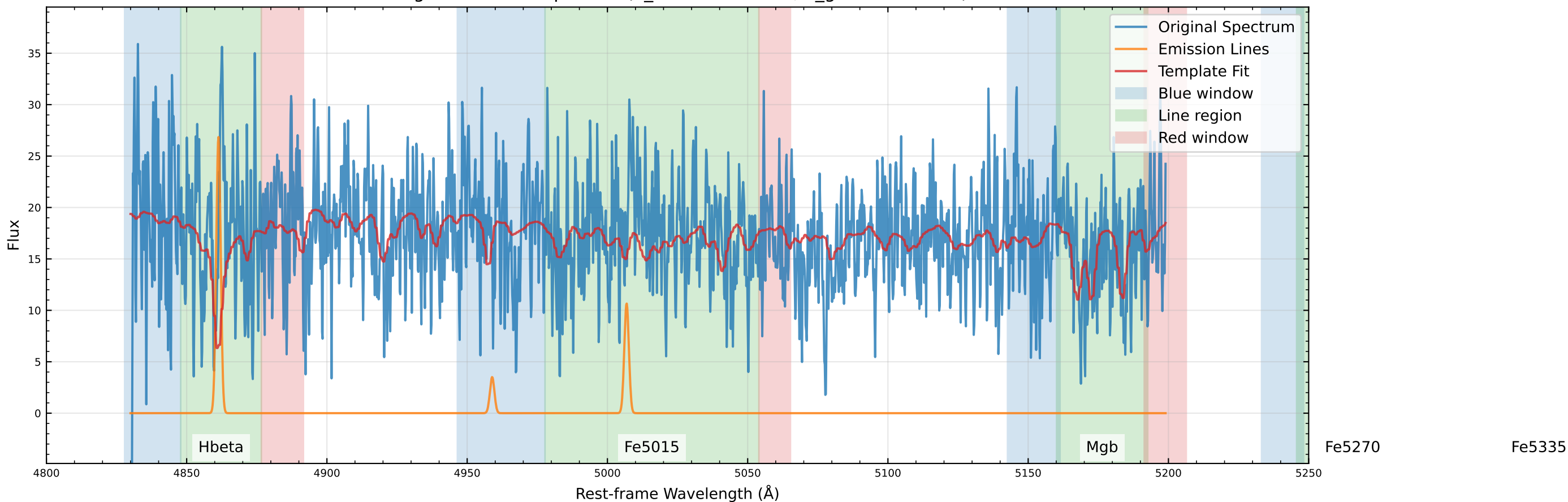
Original Data Comparison (v_star=73.4 km/s, v_gas=72.4 km/s)
