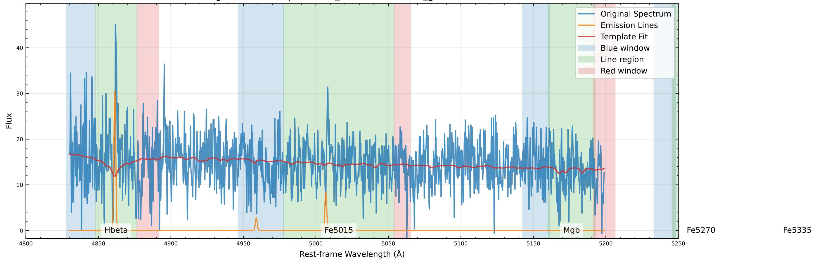
Original Data Comparison (v_star=59.0 km/s, v_gas=54.9 km/s)
