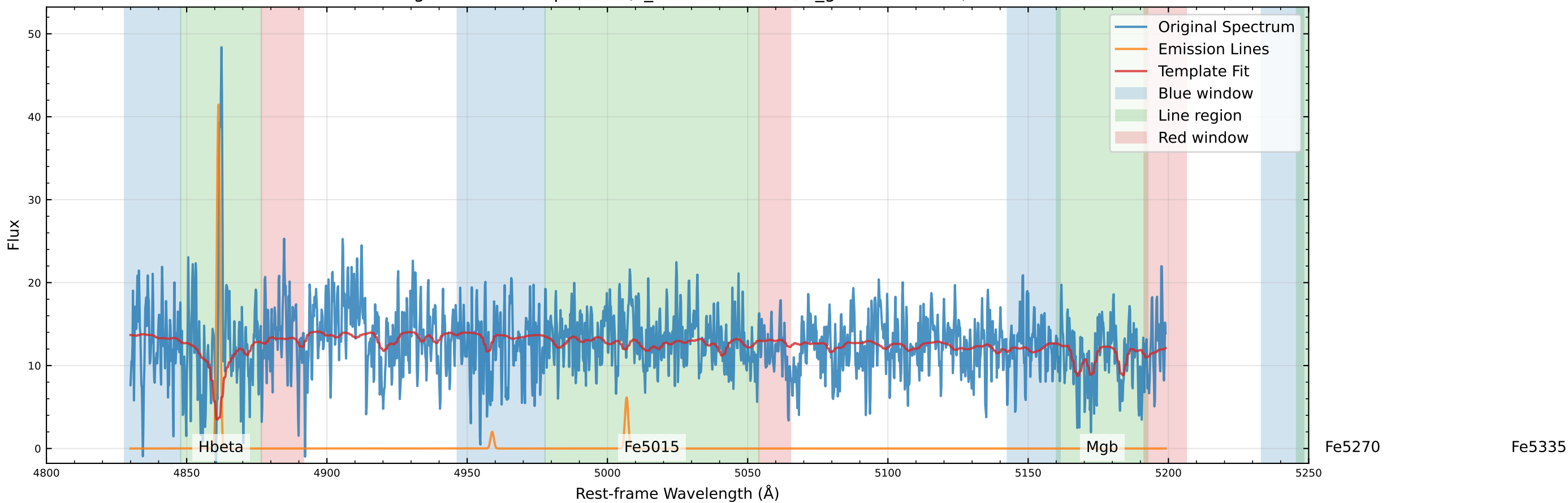
Original Data Comparison (v_star=18.0 km/s, v_gas=48.7 km/s)
