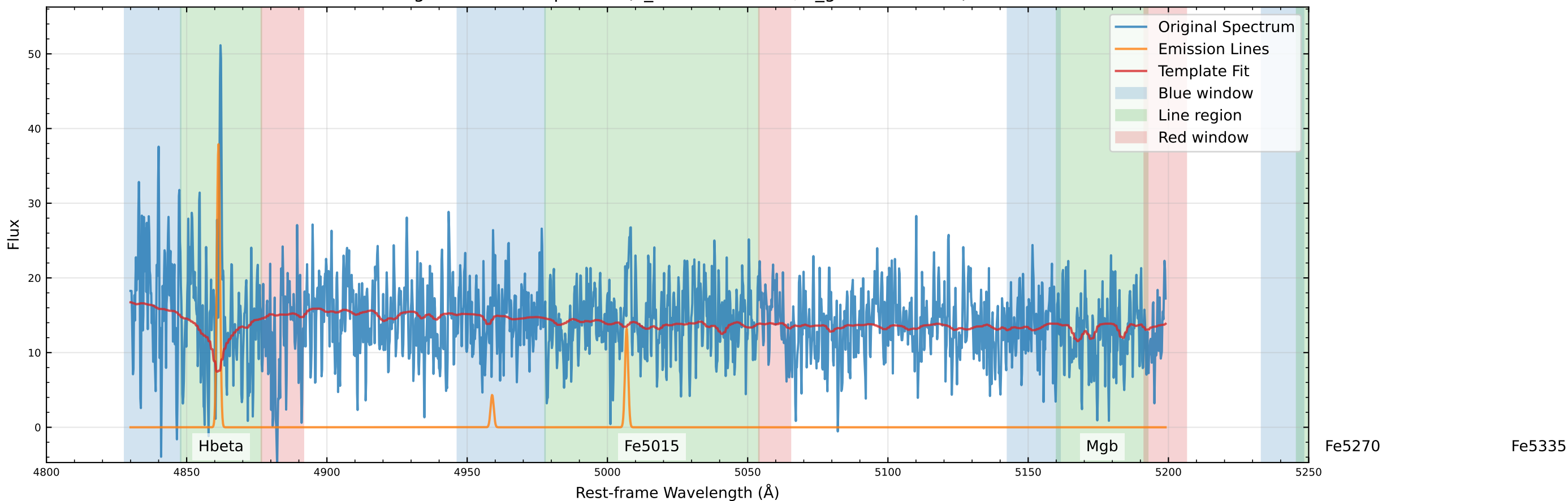
Original Data Comparison (v_star=47.0 km/s, v_gas=46.7 km/s)
