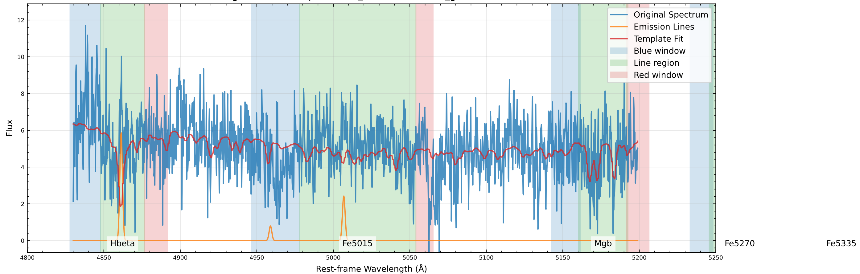
Original Data Comparison (v_star=7.4 km/s, v_gas=-6.1 km/s)
