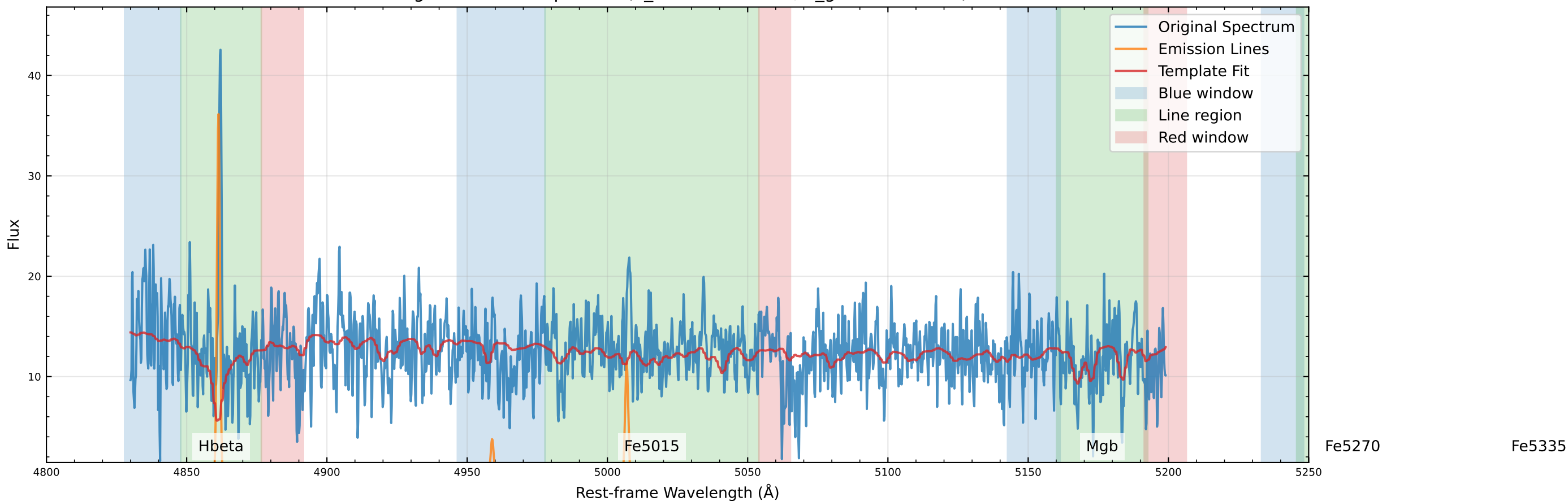
Original Data Comparison (v_star=38.4 km/s, v_gas=37.2 km/s)
