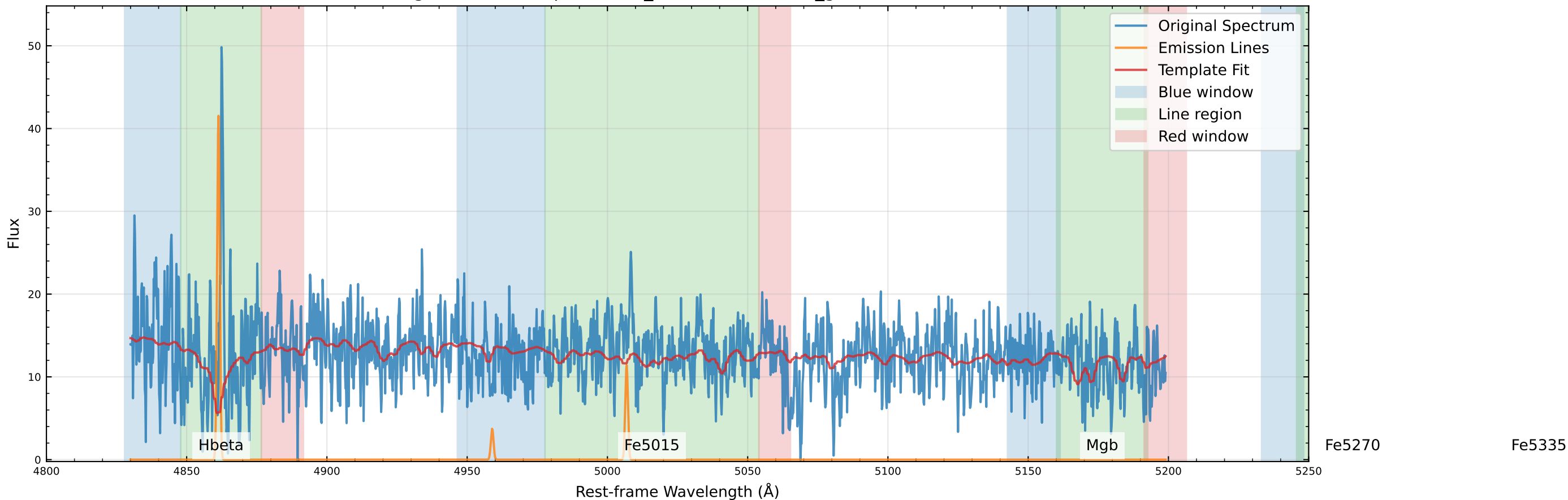
Original Data Comparison (v_star=71.9 km/s, v_gas=77.7 km/s)
