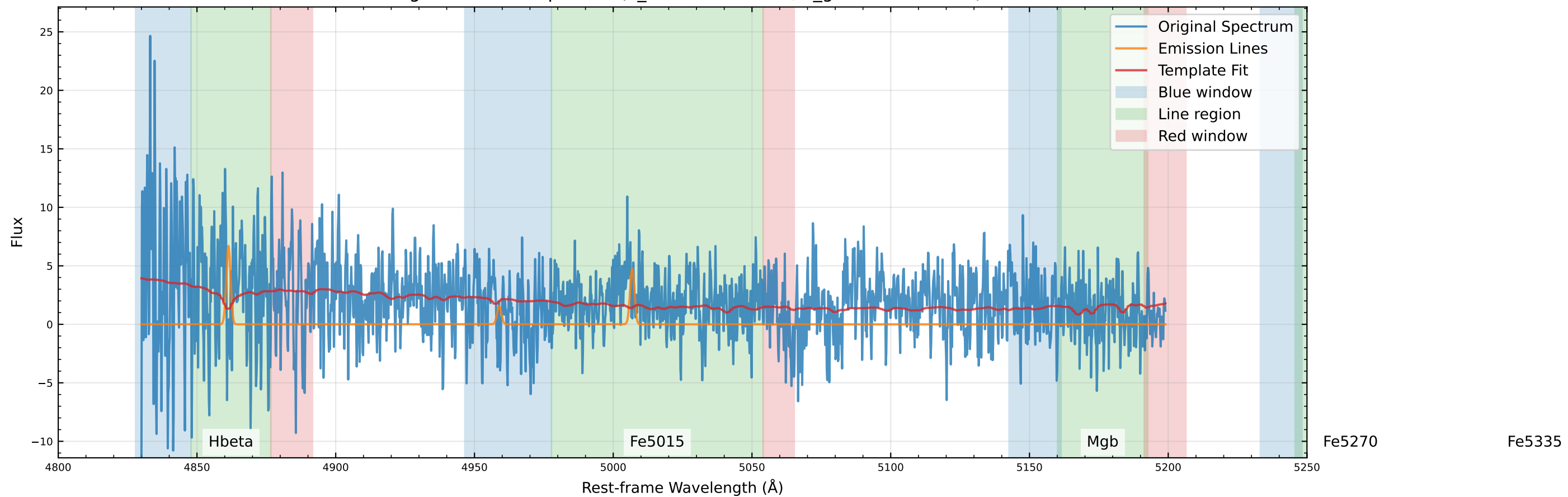
Original Data Comparison (v_star=-80.6 km/s, v_gas=-114.8 km/s)
