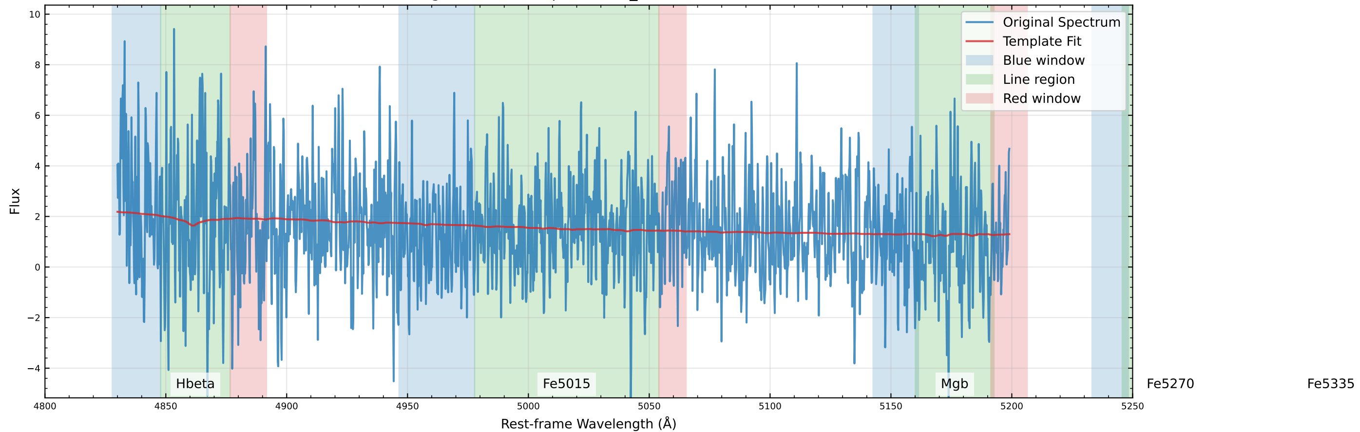
Original Data Comparison (v_star=-56.1 km/s)
