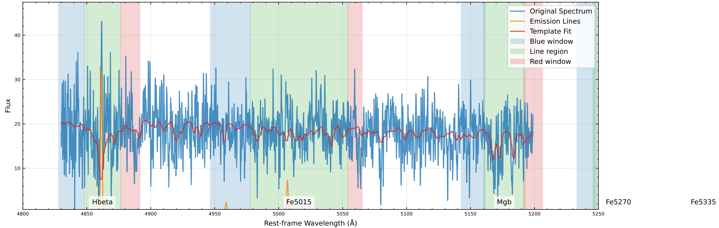
Original Data Comparison (v_star=-34.7 km/s, v_gas=1.1 km/s)
