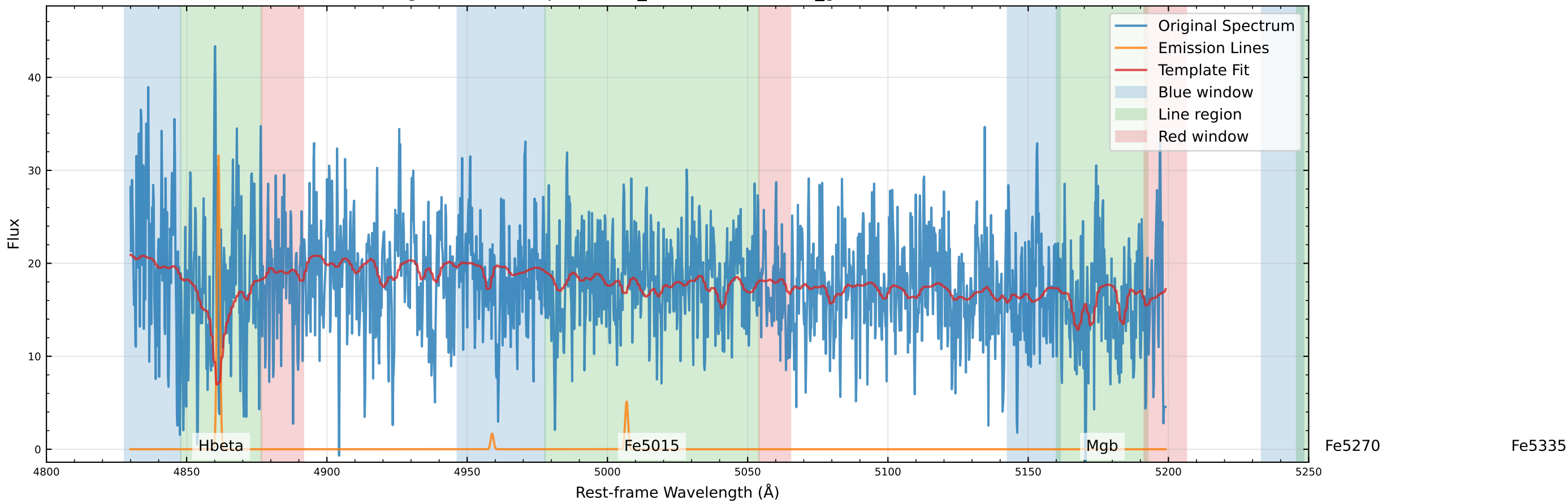
Original Data Comparison (v_star=-68.8 km/s, v_gas=-73.2 km/s)
