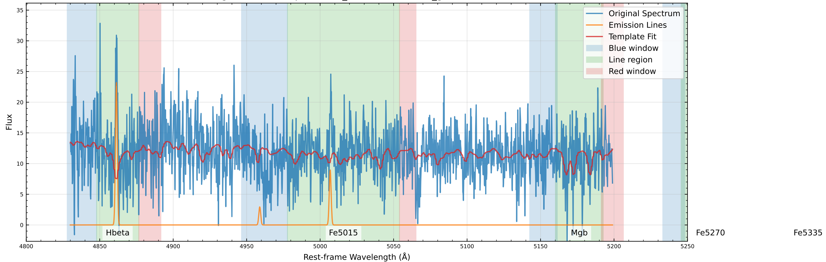
Original Data Comparison (v_star=18.0 km/s, v_gas=9.1 km/s)
