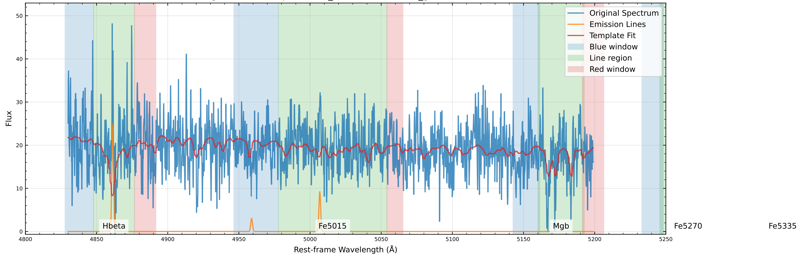
Original Data Comparison (v_star=-27.2 km/s, v_gas=-8.2 km/s)
