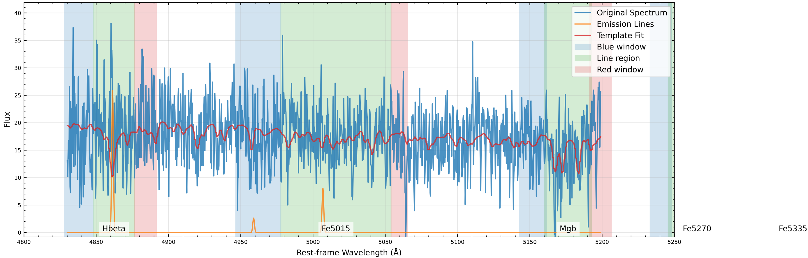
Original Data Comparison (v_star=-12.9 km/s, v_gas=-58.1 km/s)
