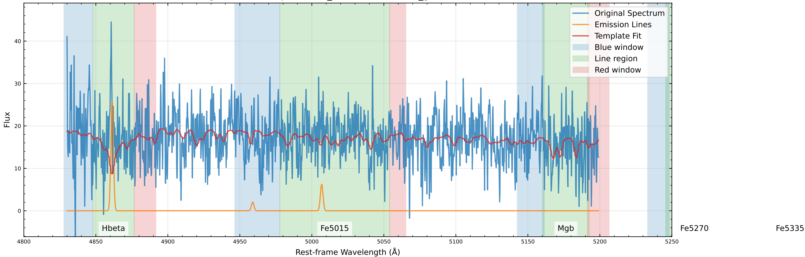
Original Data Comparison (v_star=-33.2 km/s, v_gas=-51.0 km/s)
