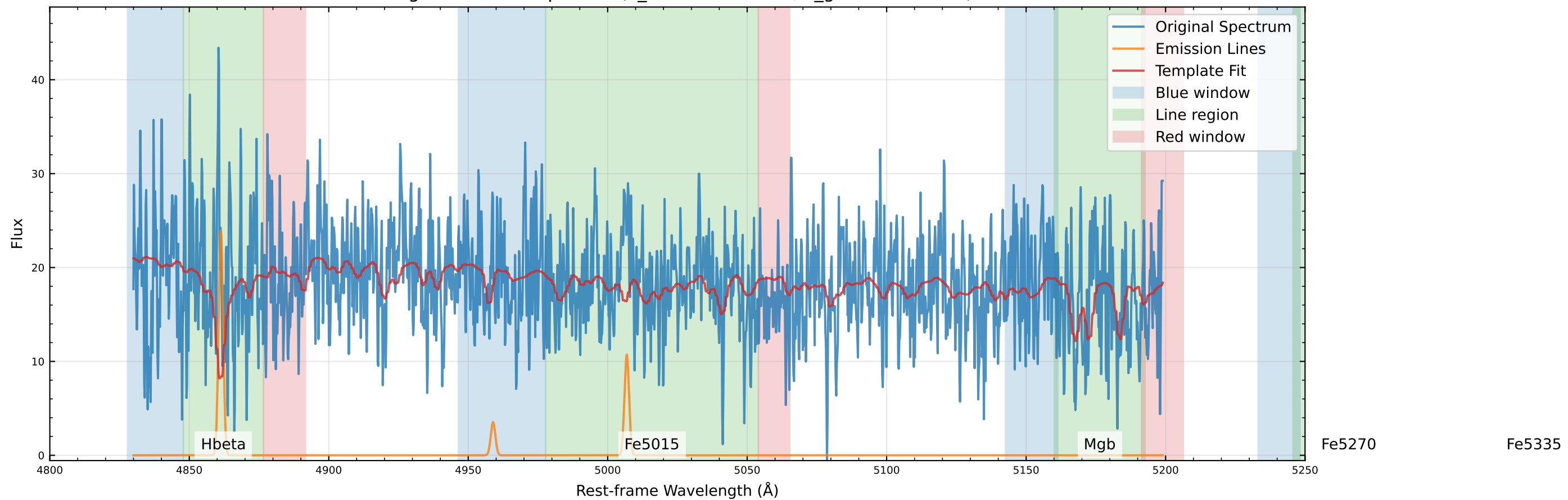
Original Data Comparison (v_star=-52.2 km/s, v_gas=-55.2 km/s)
