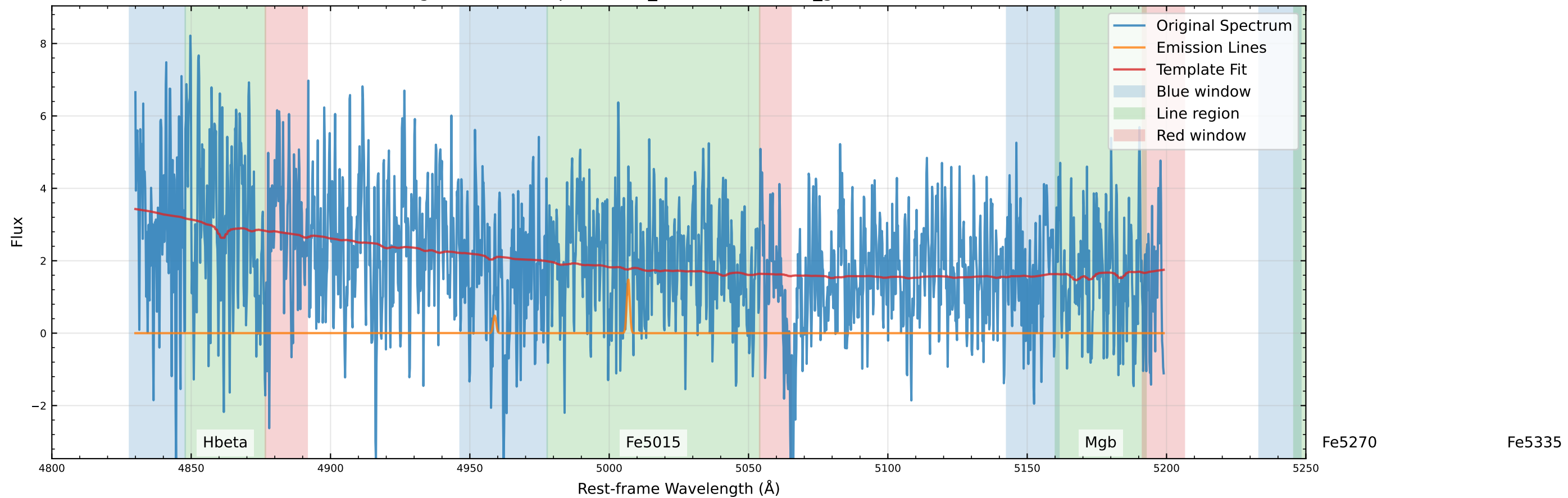
Original Data Comparison ( v_{\text{star}}=-0.4 km/s, v_{\text{gas}}=34.3 km/s)
