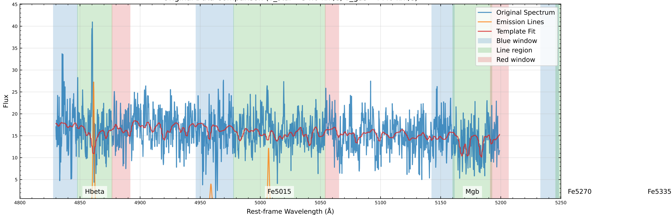
Original Data Comparison (v_star=-54.0 km/s, v_gas=-77.0 km/s)
