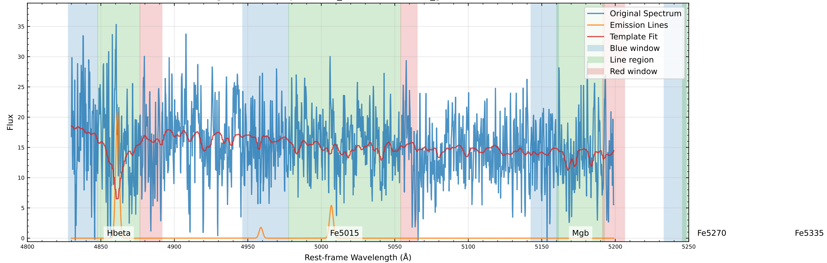
Original Data Comparison ( v_{\text{star}}=-32.3 km/s, v_{\text{gas}}=-62.8 km/s)
