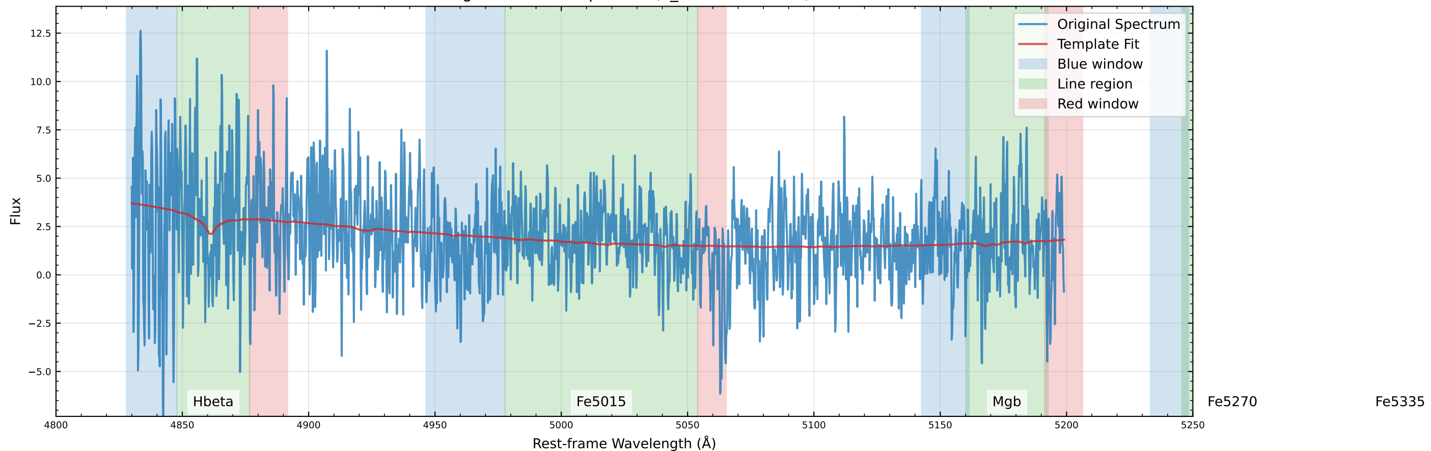
Original Data Comparison (v_star=31.3 km/s)
