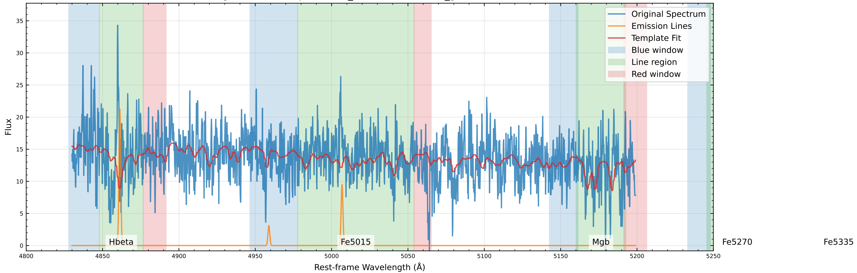
Original Data Comparison (v_star=-83.7 km/s, v_gas=-77.3 km/s)
