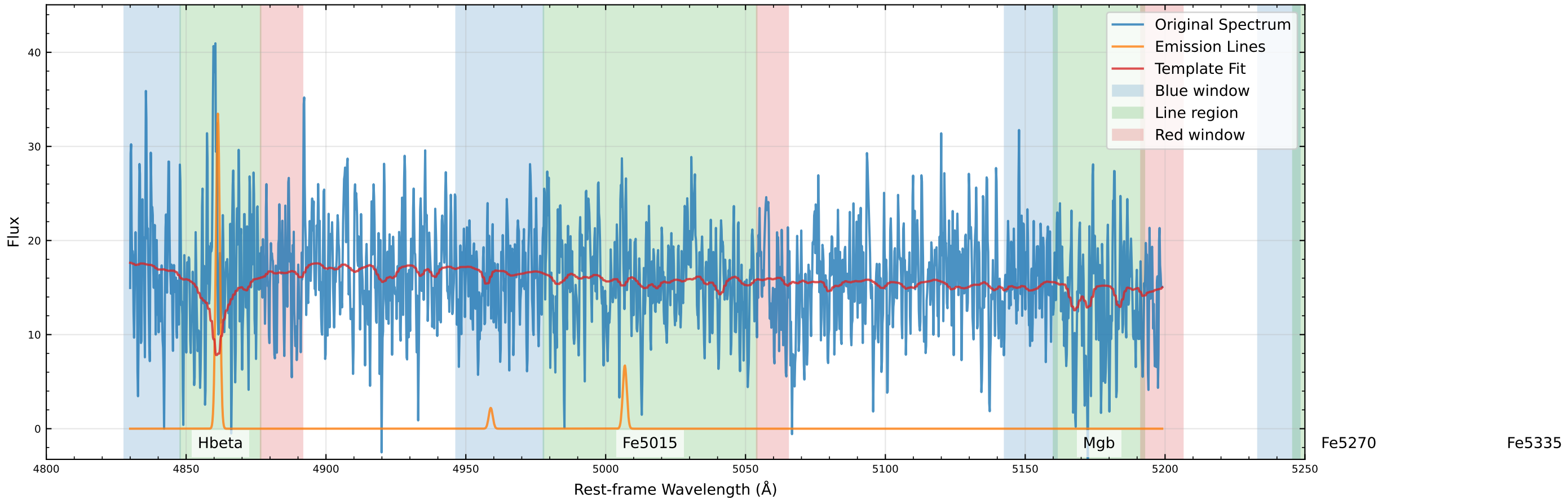
Original Data Comparison (v_star=-49.0 km/s, v_gas=-72.3 km/s)
