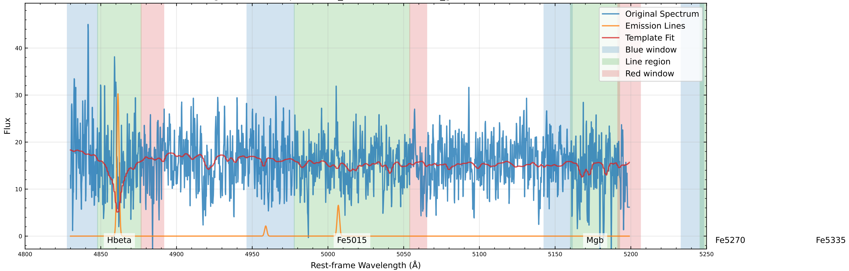
Original Data Comparison (v_star=-150.2 km/s, v_gas=-114.3 km/s)
