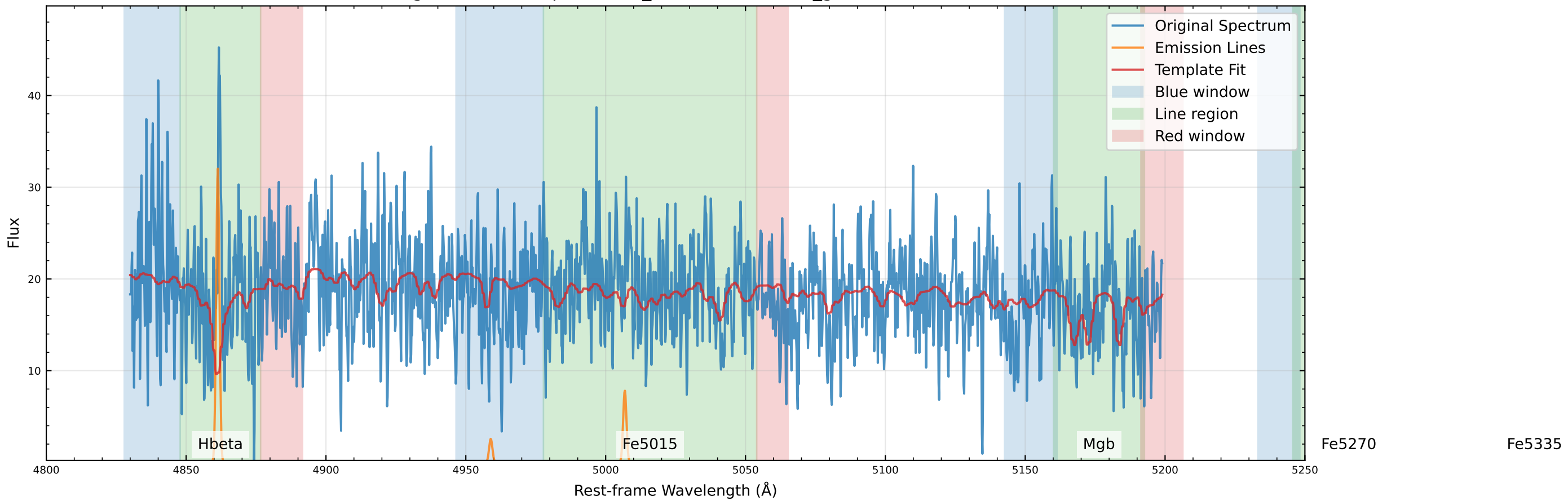
Original Data Comparison (v_star=60.4 km/s, v_gas=35.8 km/s)
